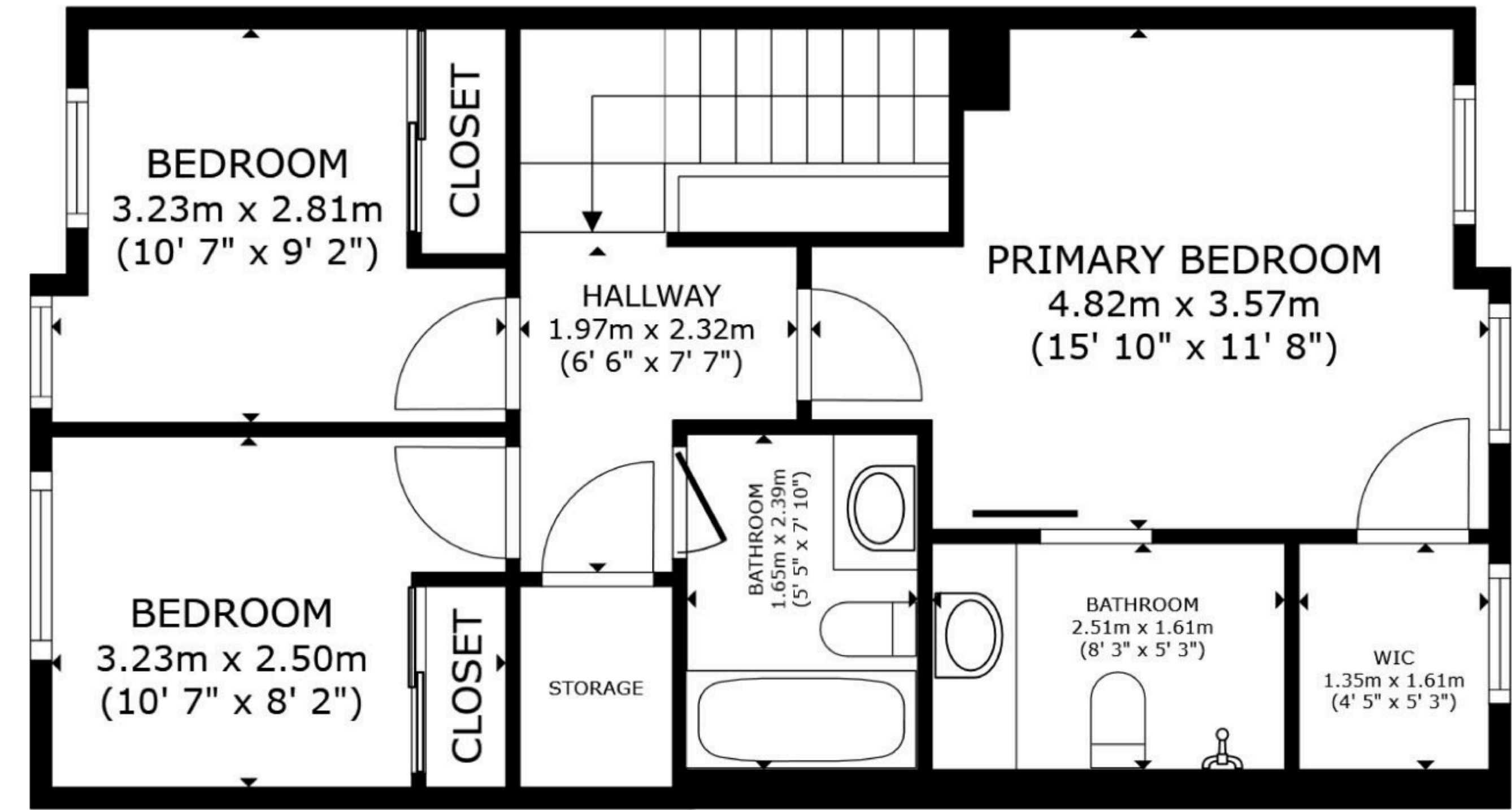
FLOOR 3
